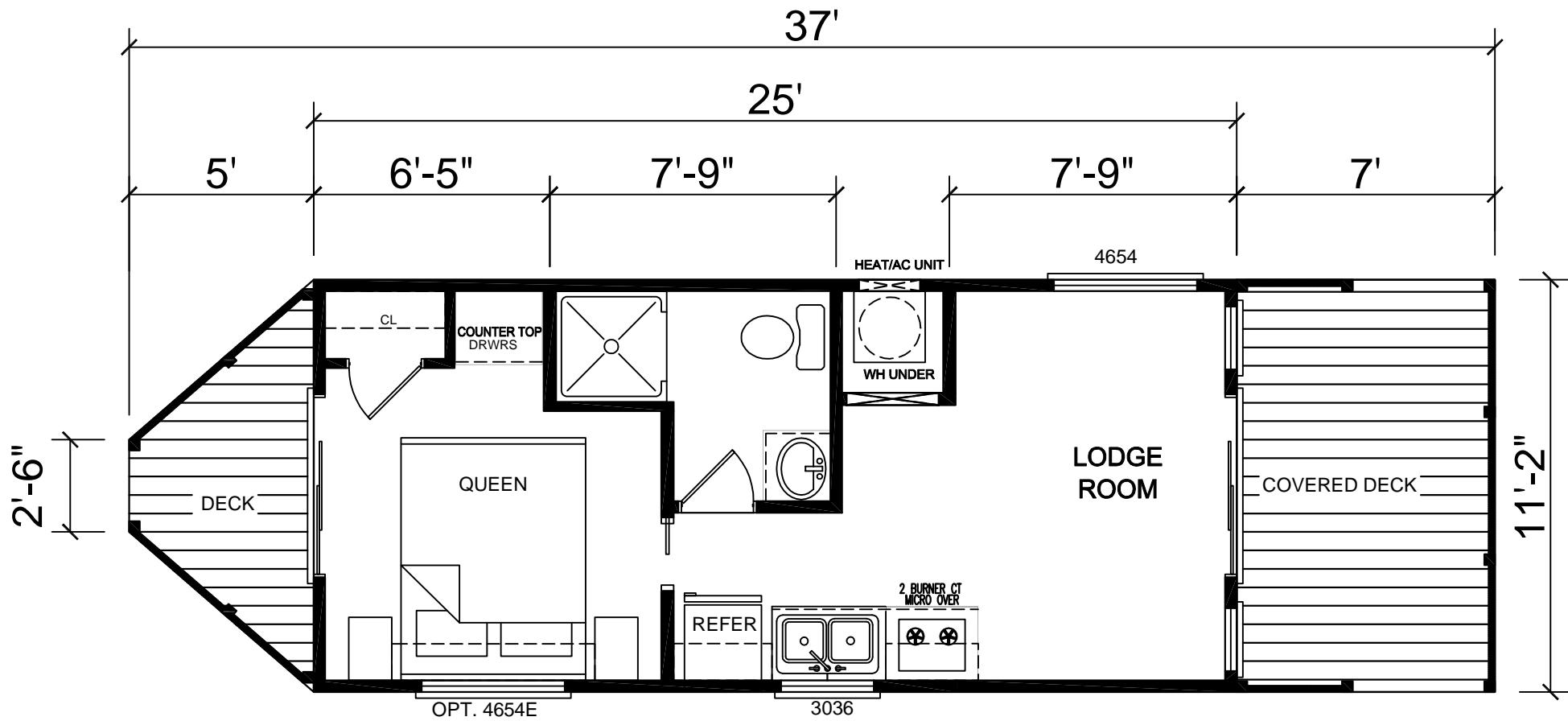
APH-1001FL 280 SF +( 112 SF DECK AS SHOWN)
