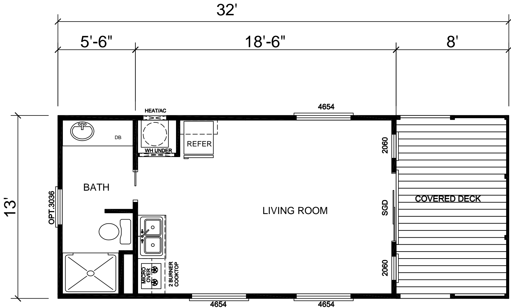
APH-1003FL 312 SQ FT W/104 SQ. FT DECK
