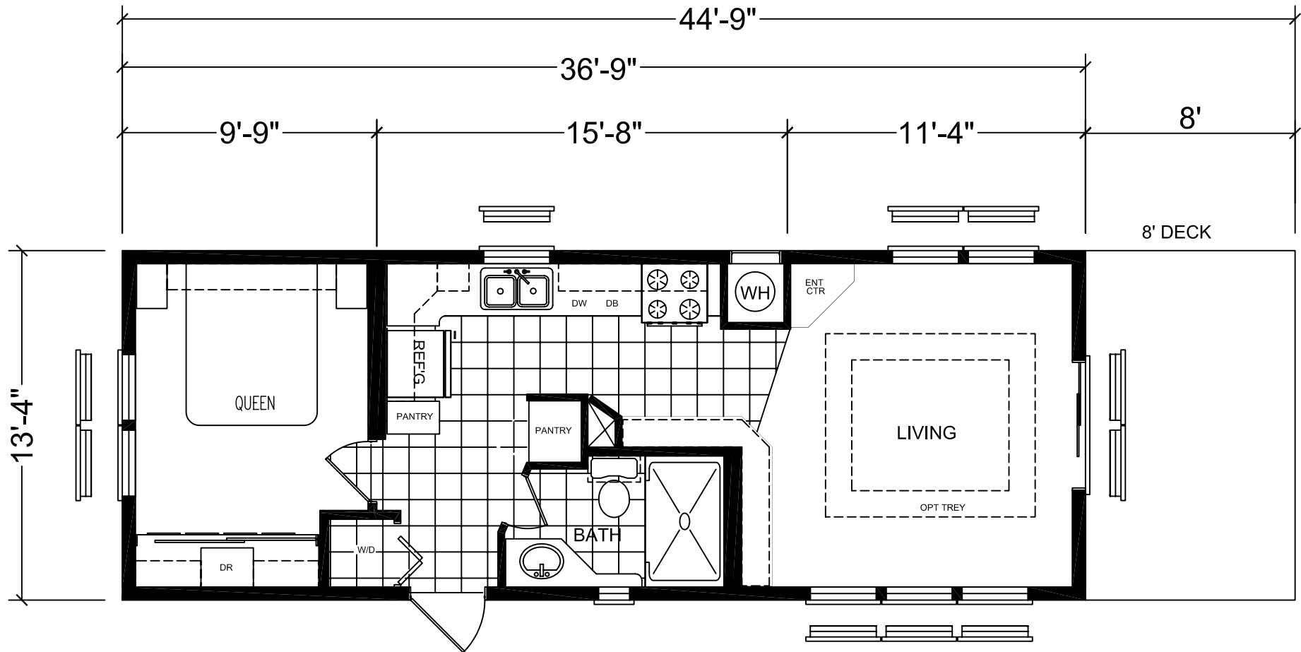
APH-HUD-607-WZIII -SPECIAL AREA= 499 SF
