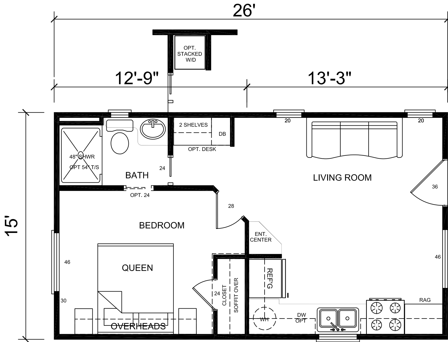
APH-460 Sportsman's Lodge 399 SQ FT
